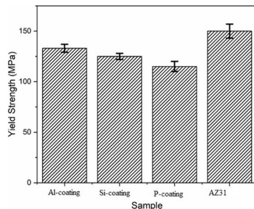
Fig. 12. Yield strength of the untreated and PEO-coated AZ31 alloy specimens in air
